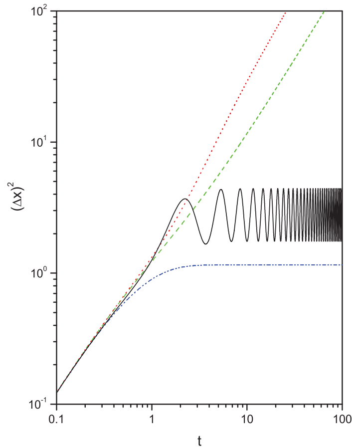
FIG. 1. (Color online) This figure illustrates Eq. (12) versus t for different time-dependent functions k(t) . The blue dashed-dotted line, which corresponds to the case k(t) = \bar{k} = \text{const.} , has a stationary value indicating the presence of a stationary solution for the system. The cases characterized by k(t) = \bar{k}/(1+t) and k(t) = \bar{k}e^{(-t)} are illustrated by the green dashed line and the red dotted line, respectively. These two cases for long time have as asymptotic behavior for the second moment a power law similar to the ones found in anomalous diffusion processes. The black solid line is the case k(t) = \bar{k} \cos^2(t) . For simplicity, in all cases we consider \eta = -1/3 , \bar{k} = 1 , and \tilde{\mathcal{D}} = 1 .
