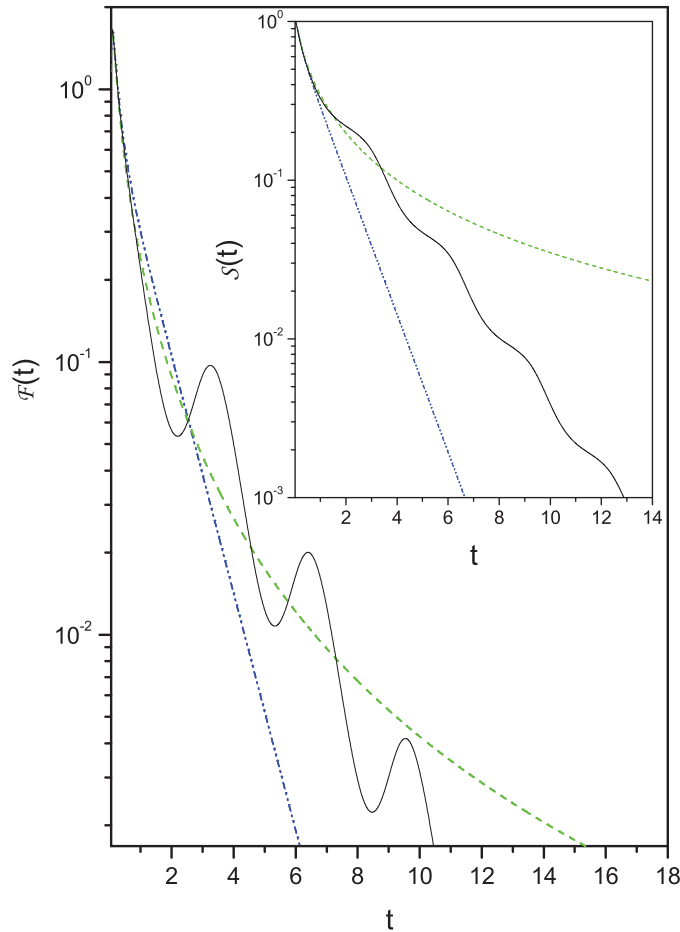
FIG. 3. (Color online) The behavior of Eq. (24) versus t for different time-dependent functions k(t) is illustrated. The blue dashed-dotted line, green dashed line, and black line correspond, respectively, to the cases k(t) = \bar{k} , k(t) = \bar{k}/(1+t) , and k(t) = \bar{k} \cos^2(t) . The inset illustrates the behavior of Eq. (23) versus t . For simplicity, in all cases we consider \eta = 1 , \bar{x} = 1 , \bar{k} = 1 , \mathcal{K} = 1 , and \mathcal{D} = 1 .
