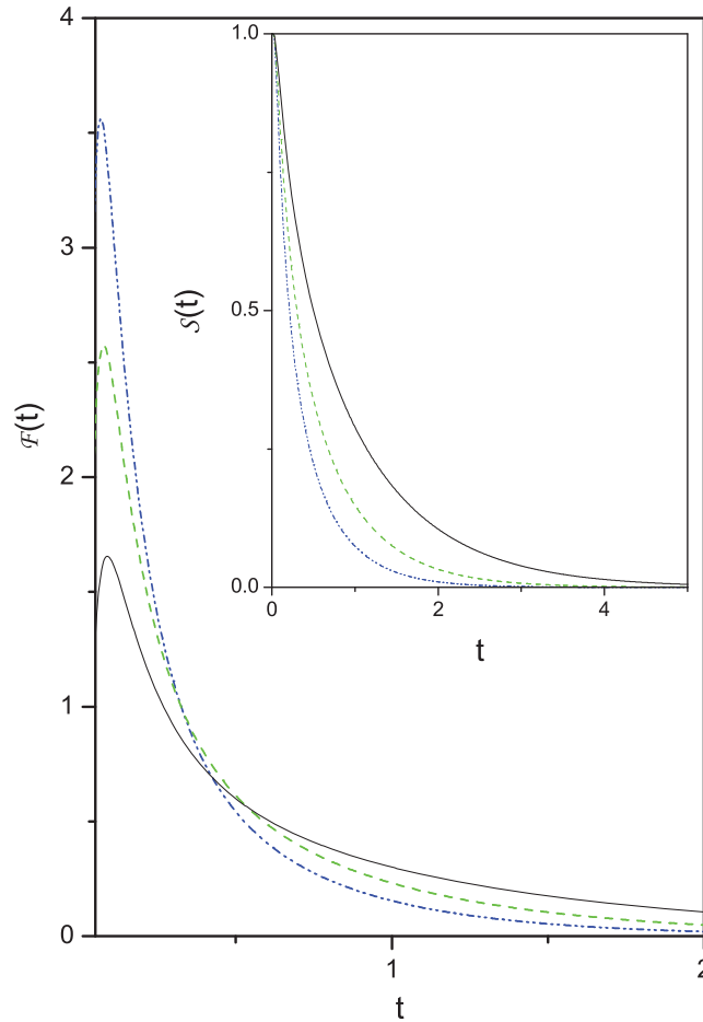
FIG. 4. (Color online) The behavior of Eq. (24) versus t for different time-dependent functions \mathcal{K} is illustrated. The blue dashed-dotted line, green dashed line, and black line correspond, respectively, to the cases \mathcal{K} = 0 , \mathcal{K} = 0.5 , and \mathcal{K} = 1.0 . The inset illustrates the behavior of Eq. (23) versus t . For simplicity, in all cases we consider \eta = 1 , \bar{x} = 1 , \bar{k} = 1 , and \mathcal{D} = 1 .
