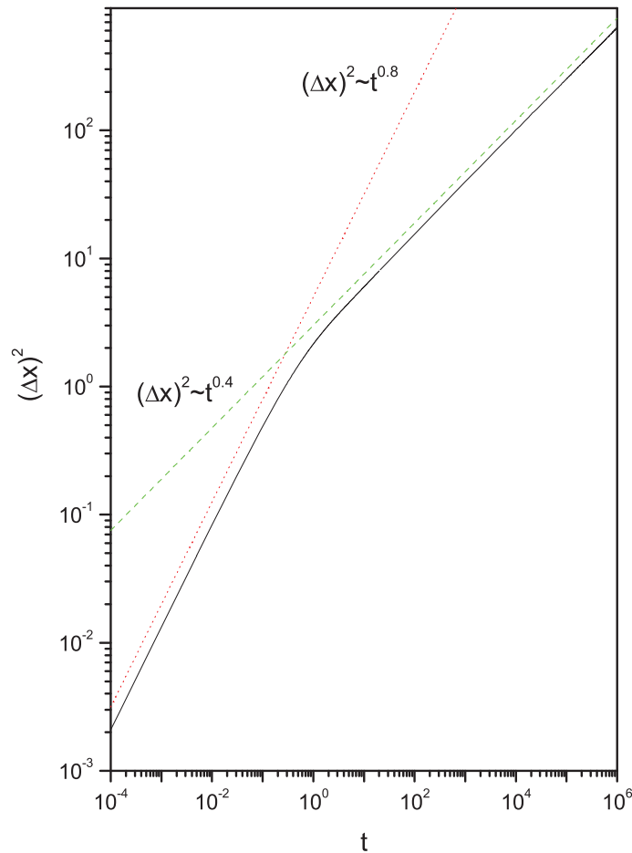
FIG. 2. (Color online) The behavior of (\Delta x)^2 versus t is illustrated, for simplicity, by considering \eta = 1/2, \bar{k} = 1, \mathcal{K} = 1, \mathcal{D} = 1 , and the initial condition \rho(x, 0) = \delta(x) . Note that the red dotted line and the dashed green line were incorporated in this figure to evidence the different diffusive regime obtained by considering k(t) = \bar{k}E_{1/2}(-t^{1/2}) .
